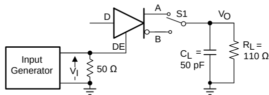
Figure 11. Measurement of Driver Enable and Disable Times With Active High Output and Pull-Down Load
