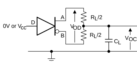
Figure 9. Measurement of Driver Differential and Common-Mode Output With RS-485 Load
