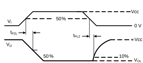
Figure 12. Measurement of Driver Enable and Disable Times With Active Low Output and Pull-up Load
