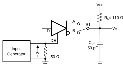
Figure 12. Measurement of Driver Enable and Disable Times With Active Low Output and Pull-up Load
