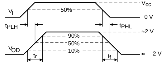
Figure 10. Measurement of Driver Differential Output Rise and Fall Times and Propagation Delays
