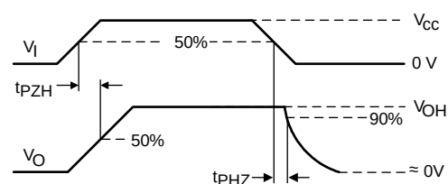
Figure 11. Measurement of Driver Enable and Disable Times With Active High Output and Pull-Down Load
