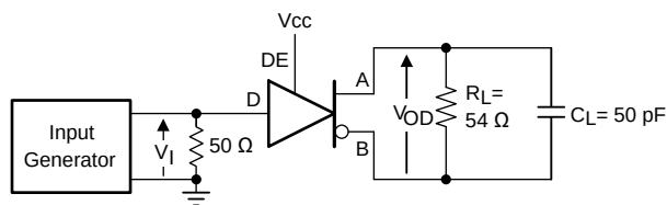
Figure 10. Measurement of Driver Differential Output Rise and Fall Times and Propagation Delays
